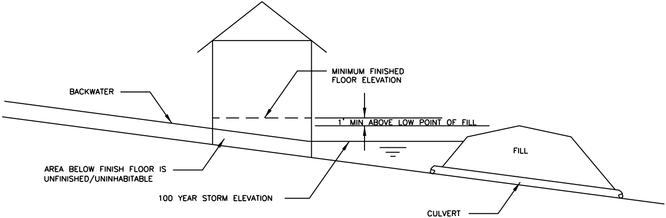
MINIMUM FINISHED FLOOR ELEVATION OF STRUCTURE LOCATED UPSTREAM OF FILL SECTION WHEN 100 YEAR STORM DOES NOT OVERTOP FILL FIGURE G-1(A)
